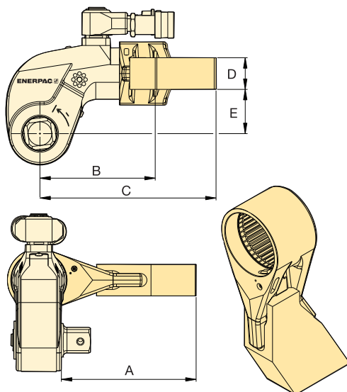
SRSX Series
