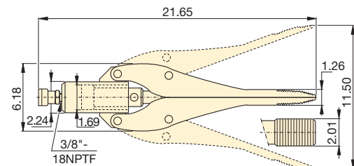
WR-15
